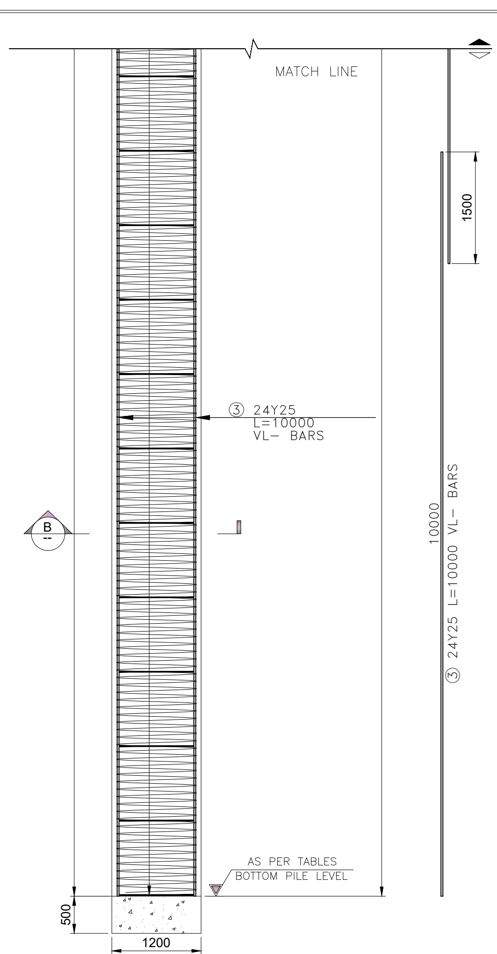
SEC ELEVATION SHOWING PILE REINFORCEMENT DETAILS 1200 MM PILE SCALE 1:50
